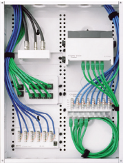
WIRING ENCLOSURES
